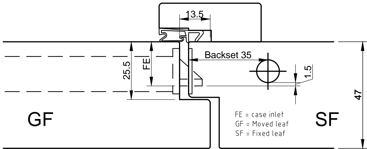
Rebate retracting bolt, locks automatically in upper and lower positions
