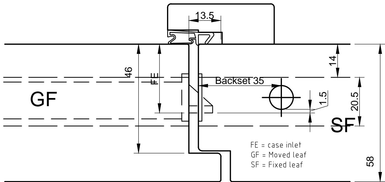
Rebate retracting bolt, locks automatically in upper and lower positions
